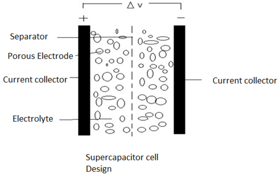
Figure 4: Schematic sketch of an electrical double layer capacitor
