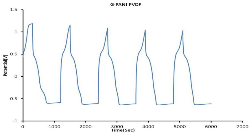
Figure 45: Charge discharge curves for G-PANI PVDF at 1 mA charging and discharging currents
